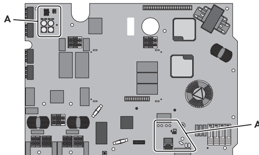
Figure 2 : Position of the SELV circuits
