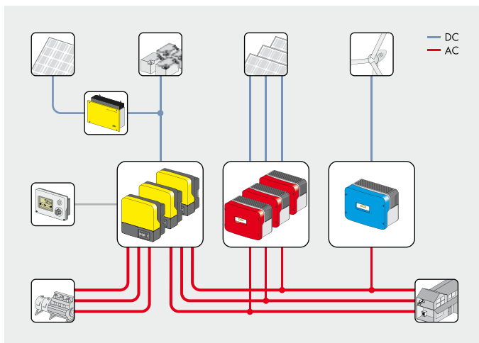
Three-phase system
