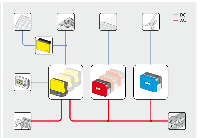
Single-phase system
