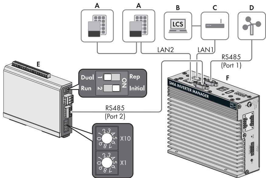
Figure 2: Circuitry Overview of Sunny Tripower 60 / Sunny Highpower 75
