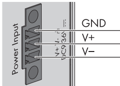
Figure 7: Pin assignment of the pin connector "Power Input" SMA recommends using the top-hat rail power supply available as an accessory (order number: CLCON-PWRSUPPLY)*.
