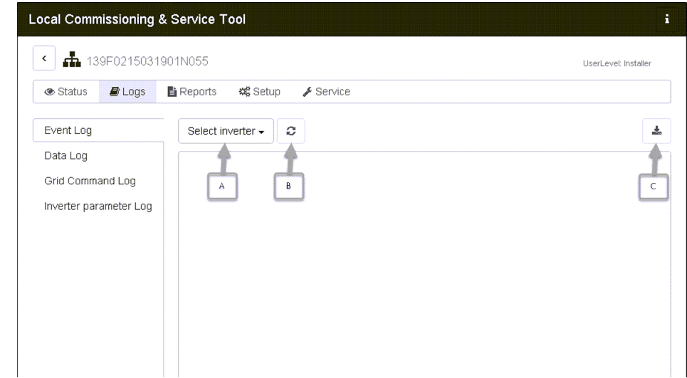
Figure 35: LCS-Tool - logs
