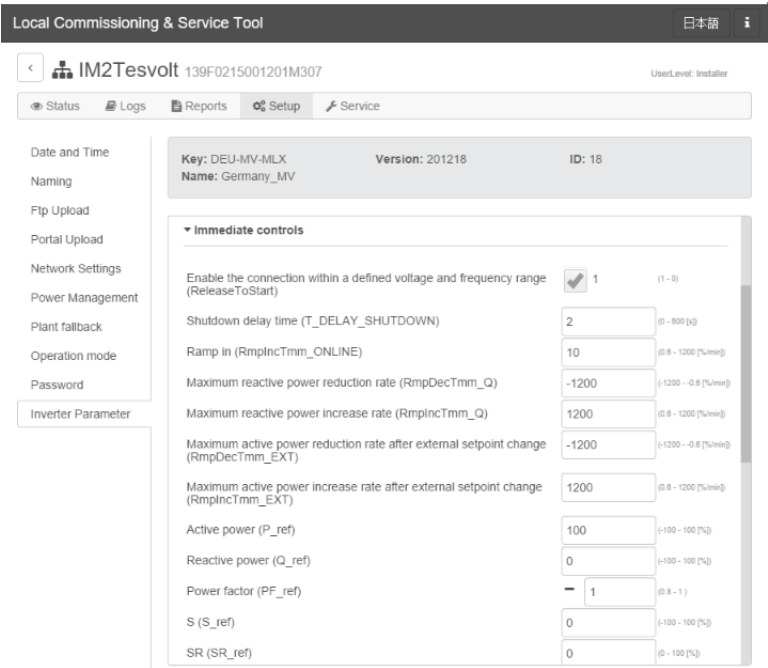
Figure 31: LCS-Tool - changing signs
