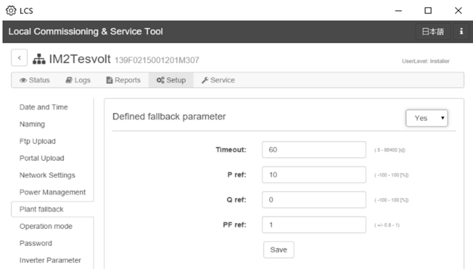
Figure 22: LCS-Tool - setting the fallback parameter
