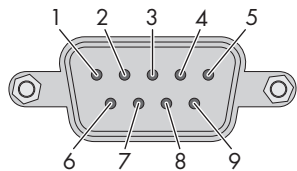
Figure 5: Pin assignment of the serial interface The I/O Box must be connected to port 2 of the Inverter Manager. Termination for the RS485 interface is not necessary.
