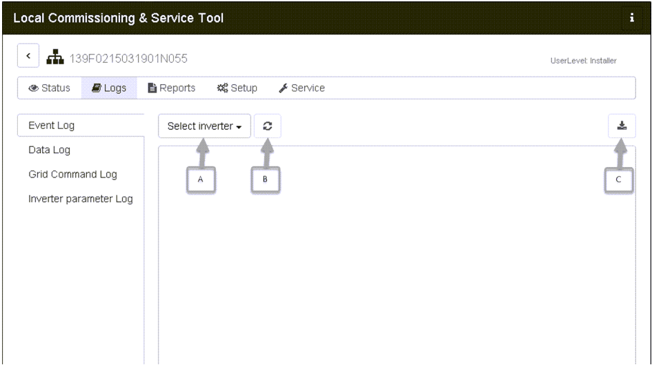
Figure 35:LCS-Tool - Logs
