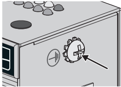
Figure 6: Position of the grounding screw Shielded ground: The shielded ground (also called "protected ground") is located at the pin connector for the electrical connection in the displayed view.
