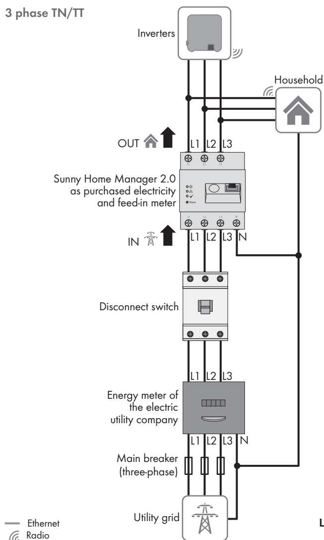
Figure 5: The following figure shows a connection example in TN and TT utility grids in the case of installation at the grid-connection point when using the integrated measuring unit.
