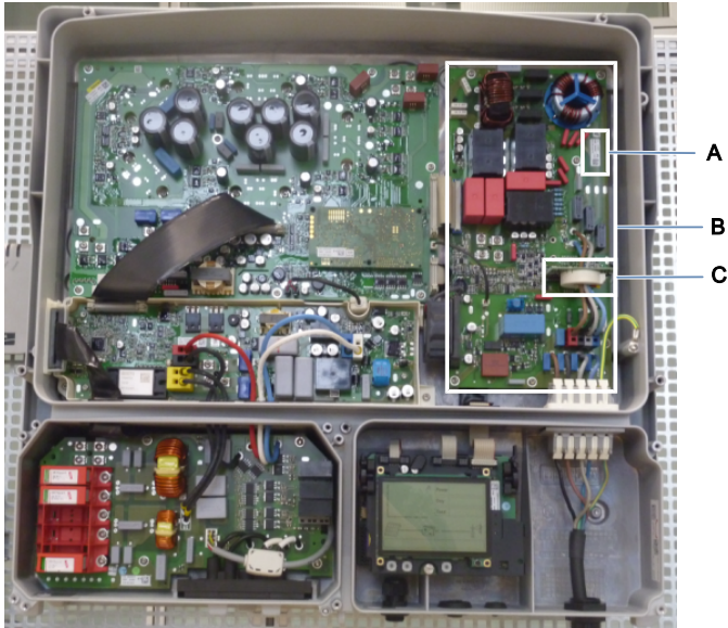
Figure 1 : Position in the inverter
